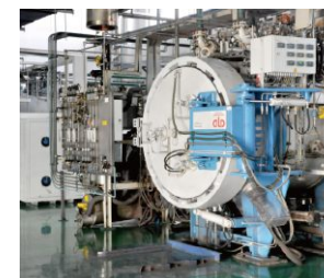
热压烧结炉 Hot Pressing Sintering Furnace
